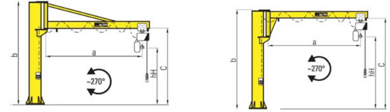
Kolonlu Pergel Vinçler Pillar Jib Cranes
