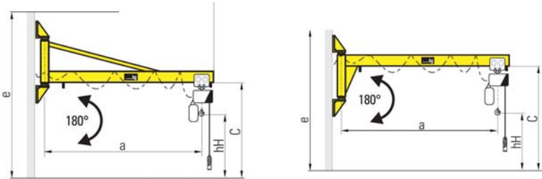
Duvara Monte Pergel Vinçler Wall-mounted Jib Cranes
